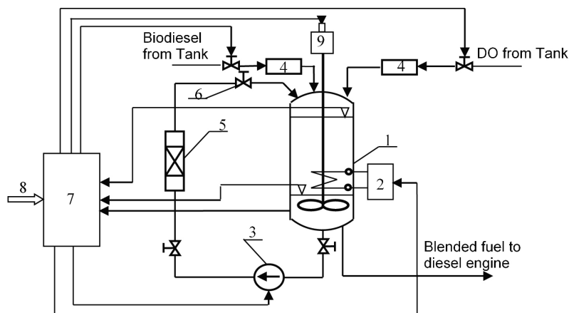
Figure 3. Fuel mixer system
