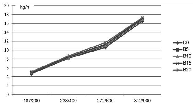
Figure 5. Fuel consumption at different loads
