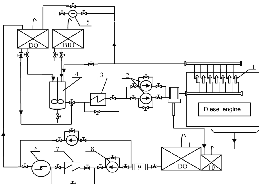
Figure 2. Modification of fuel supplying system
