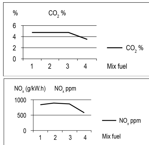
Figure 6. Emission figure when palm oil blends used
