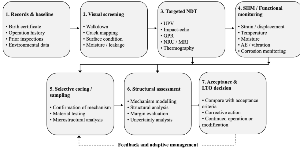
Figure 2. Evidence-based assessment and long-term-operation decision framework: GPR - Ground-Penetrating Radar; NRU/MRI - Nonlinear Resonant Ultrasound/Magnetic Resonance Imaging; AE - Acoustic Emission
