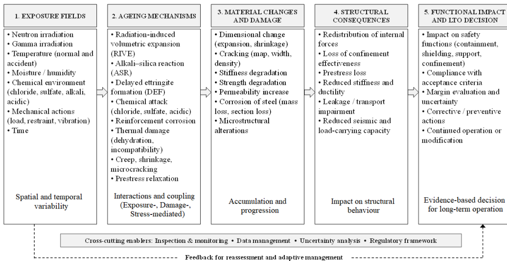
Figure 1. Coupled ageing and structural-consequence framework for concrete in nuclear power plants
