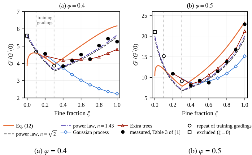
Figure 7. External test on Table 3 of [1] ( \lambda = 3.94 ; \varphi_m from Eq. (3); machine learning models trained on the 70 points of Table 1): relative modulus against the fine fraction at (a) \varphi = 0.4 and (b) \varphi = 0.5 ; dotted lines mark the training gradings
