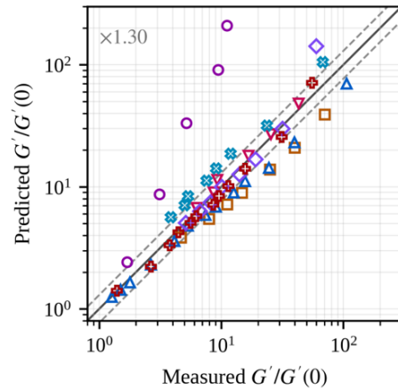
(b) Constrained symbolic regression search under leave-one-mixture-out; four points lie outside the axes
