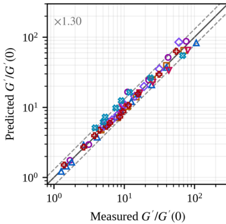
(a) Gaussian process under leave-one-mixture-out validation
