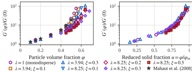
(a) Versus the particle volume fraction, together with the data of [7]
