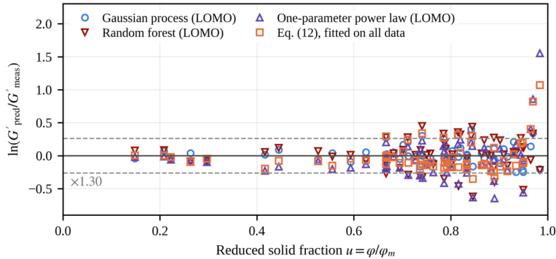
Figure 6. Logarithmic error of four models against the reduced solid fraction for the 63 measurements (normalization points at \varphi = 0 not shown); dashed lines bound the factor-of-1.30 band
