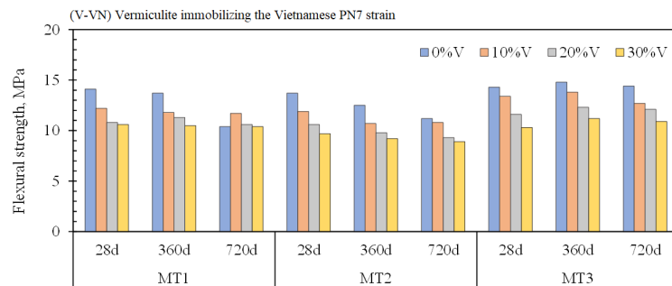
Figure 5. Flexural strength of V-VN samples under MT1, MT2, and MT3
