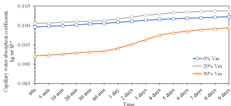
Figure 11. Capillary water absorption coefficient of samples containing PN7-immobilized vermiculite
