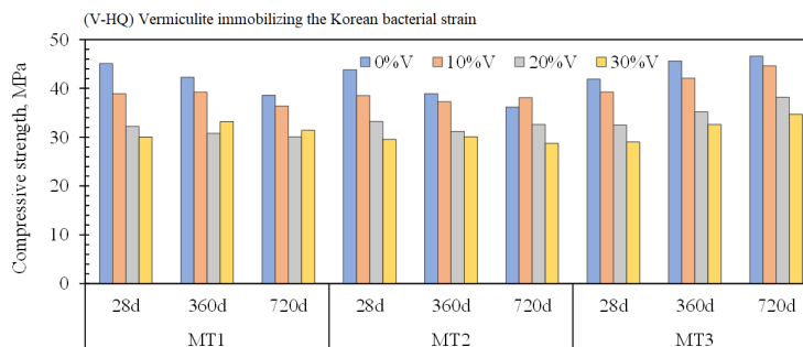
Figure 7. Compressive strength of V-HQ samples under MT1, MT2, and MT3
