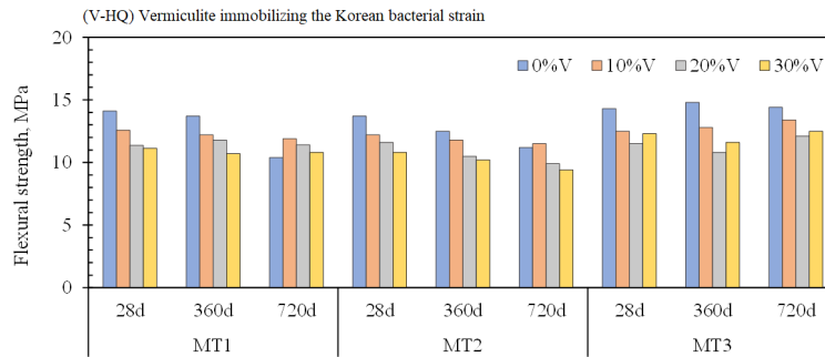
Figure 4. Flexural strength of V-HQ samples under MT1, MT2, and MT3
