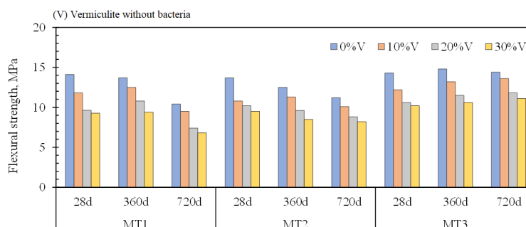
Figure 3. Flexural strength of V-samples under MT1, MT2, and MT3
