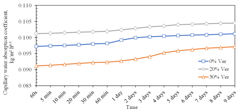
Figure 10. Capillary water absorption coefficient of samples containing vermiculite without bacteria
