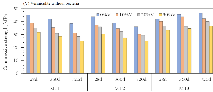
Figure 6. Compressive strength of V samples under MT1, MT2, and MT3
