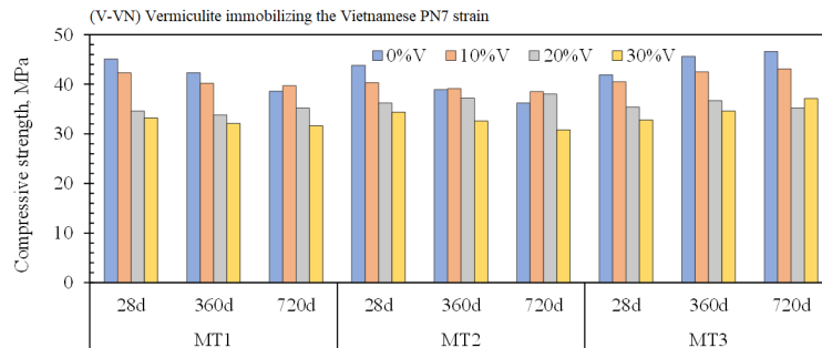
Figure 8. Compressive strength of V-VN samples under MT1, MT2, and MT3
