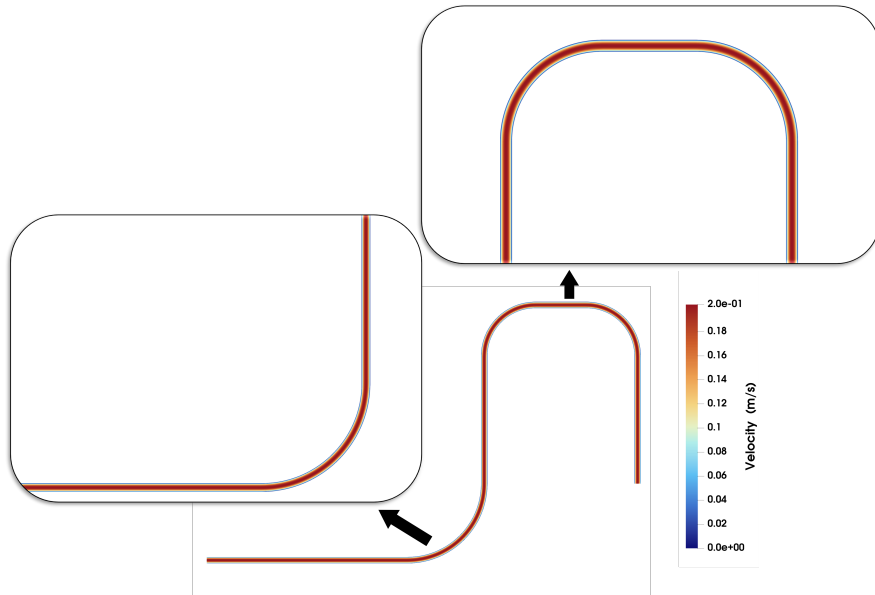
Figure 9. Simulated velocity profile of mix FIN 10 within the pumping pipe
