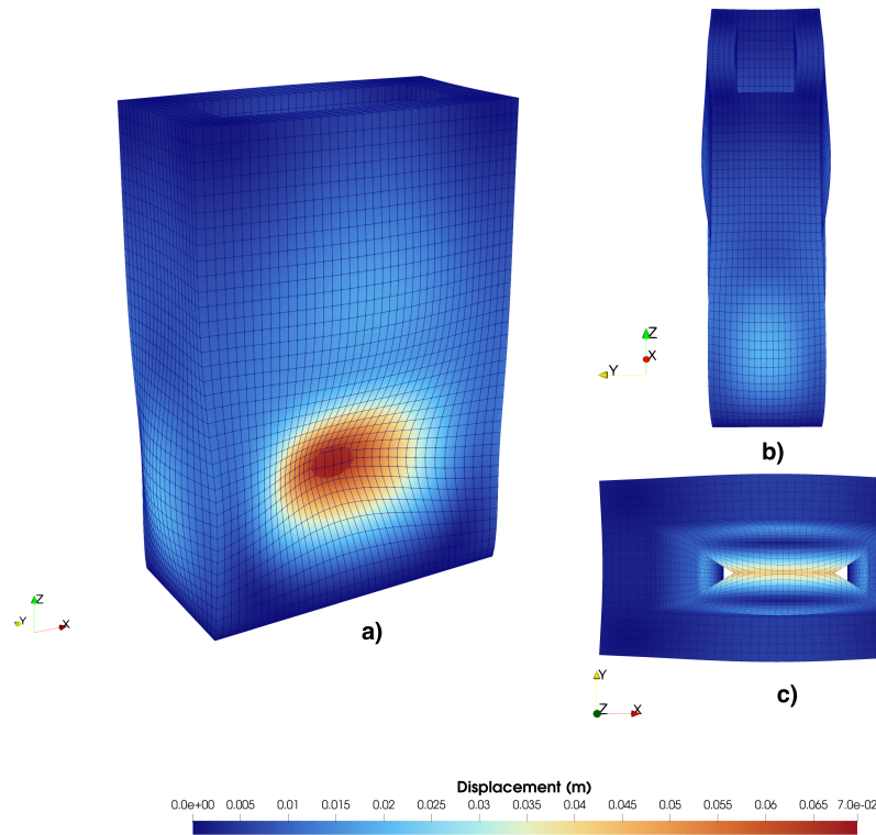
Figure 15. Displacement magnitude ( U , m) at the critical 37-layer height: isometric view (a), front view (b), and plan view (c)
