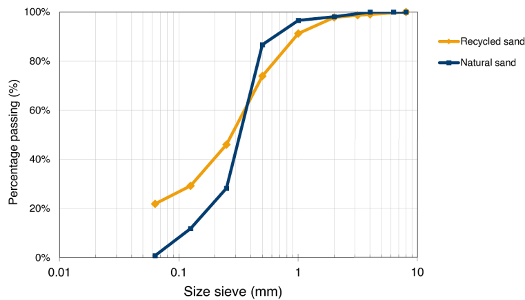
Figure 2. Particle size distribution of sand
