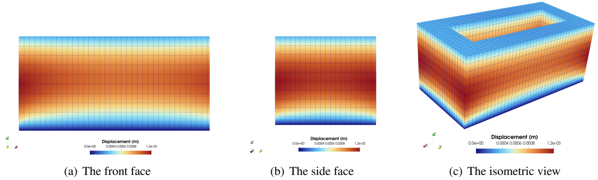
Figure 12. Displacement magnitude (U Magnitude, m) of the printed wall at layer 10, shown from the front face (a), side face (b), and isometric view (c)
