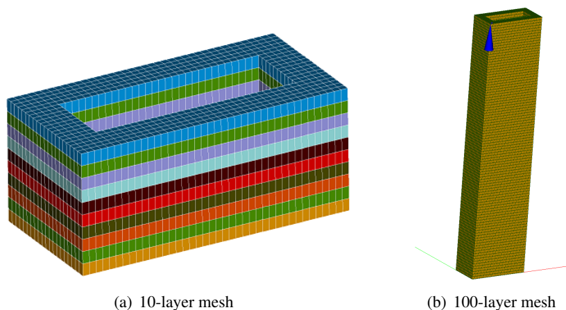
Figure 11. SALOME mesh of the printed wall: (a) 10-layer mesh, and (b) 100-layer mesh, both grouped into individual layer-wise element sets for sequential activation
