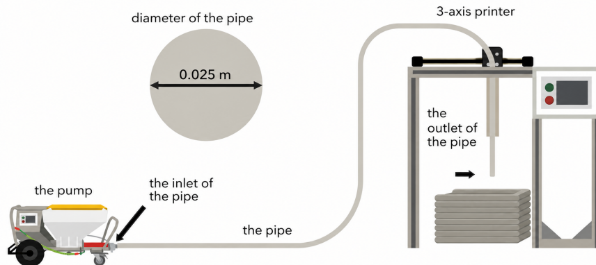
Figure 7. Geometry of the pumping pipe system, including the pump, pipe diameter, and printer nozzle outlet
