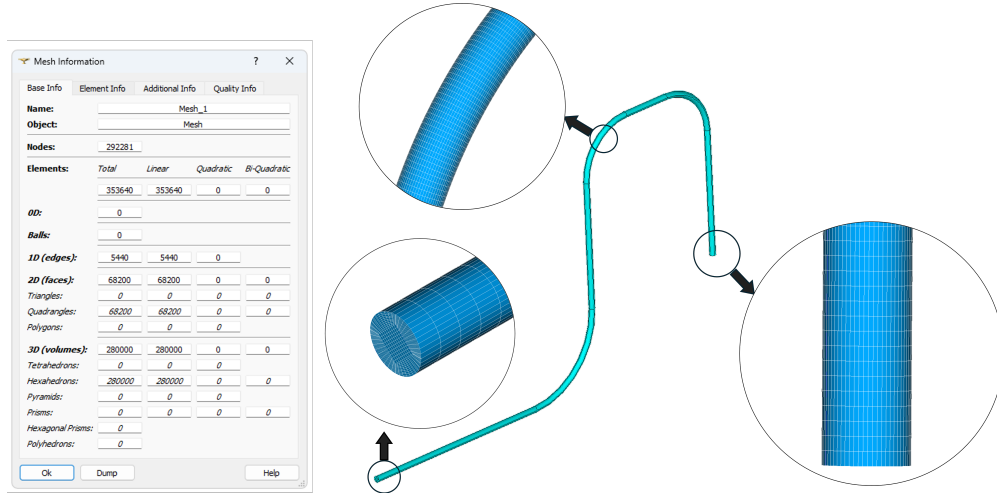
Figure 8. Mesh detail and mesh information of the pipe
