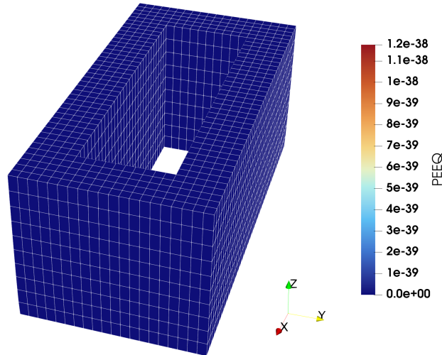
Figure 13. Equivalent plastic strain (PEEQ) contours at layer 10
