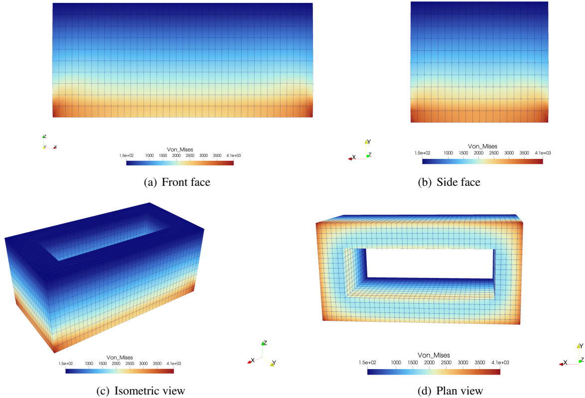
Figure 14. Von Mises stress (Von_Mises, Pa) contours of the printed wall at layer 10: front face (a), side face (b), isometric view (c), and plan view (d)
