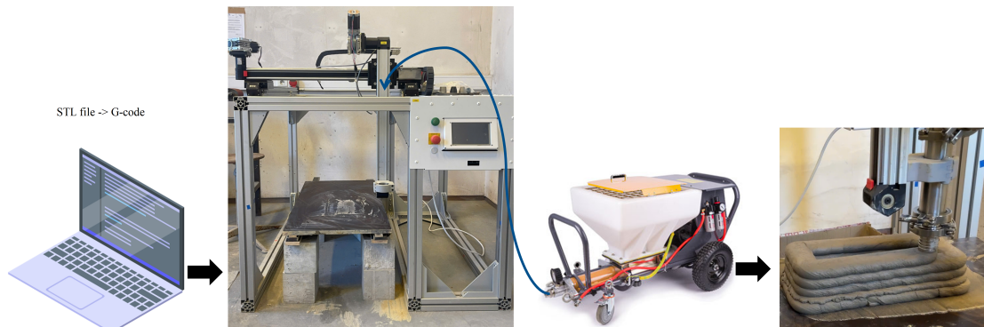
Figure 3. The 3D printing process: STL file converted to G-code, 3-axis gantry printer, material pump, and layer-by-layer deposition of the mortar
