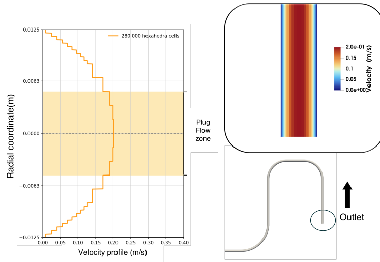
Figure 10. Velocity profile at the outlet
