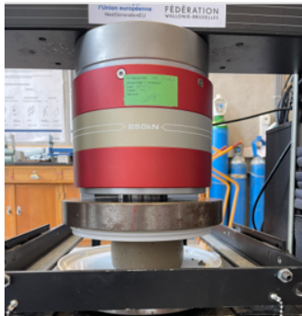
(a) Compression platen and specimen
