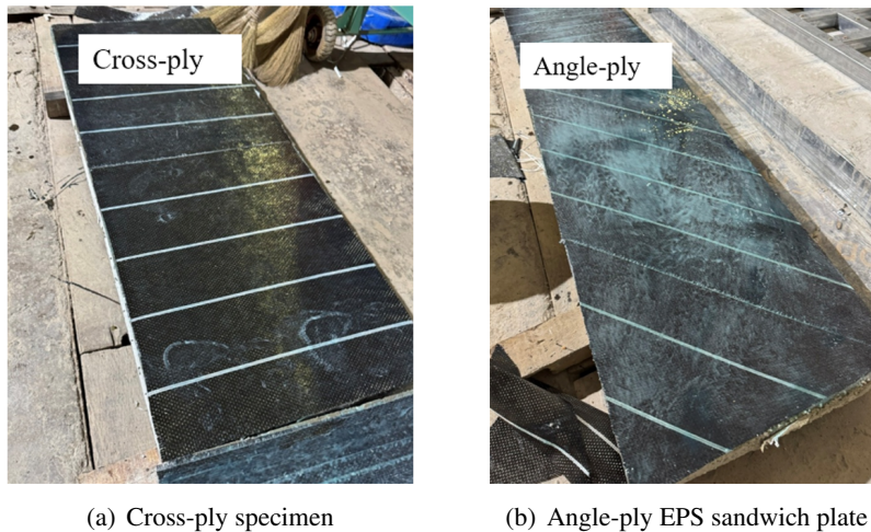
Figure 4. Specimens
