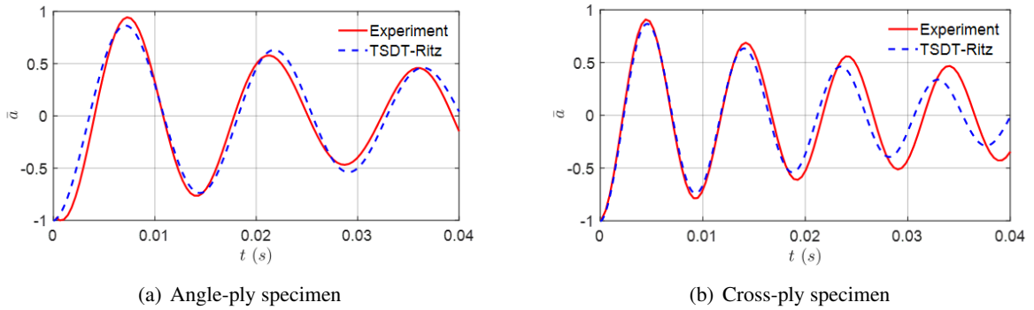
Figure 8. Acceleration-time history at the plate center
