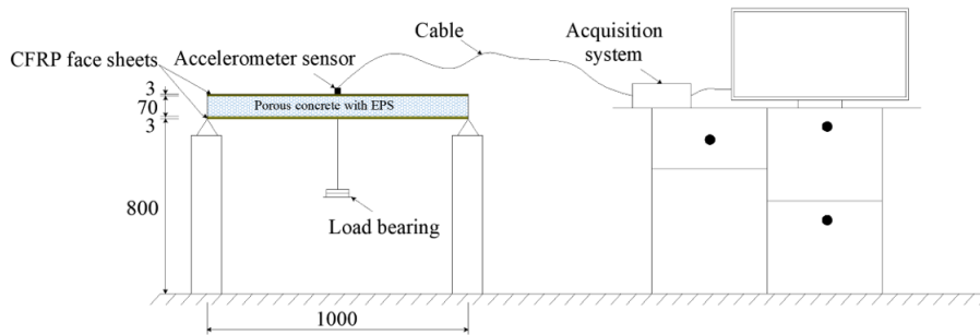
Figure 5. Schematic of the vibration test setup (unit: mm)
