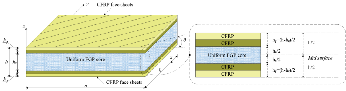
Figure 1. Sandwich plate geometry and coordinate system
