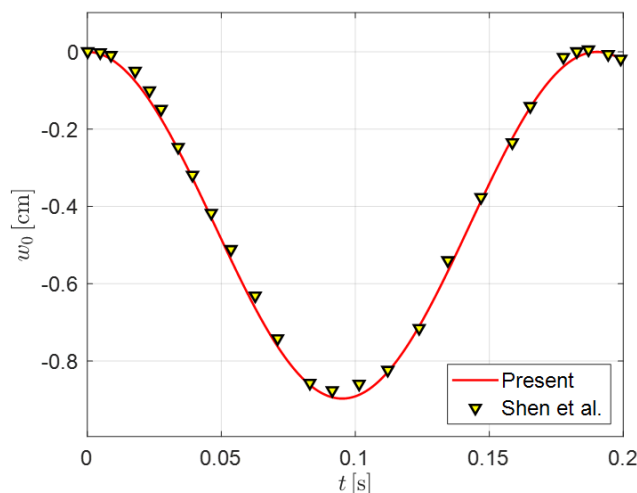
Figure 2. Central deflection history: comparison with Shen et al. [28]
