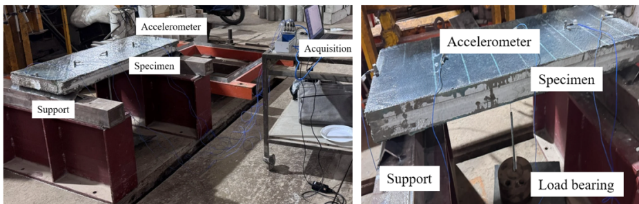
Figure 6. Installed plate and accelerometer layout
