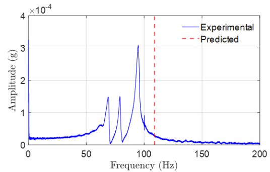
(b) Cross-ply specimen
