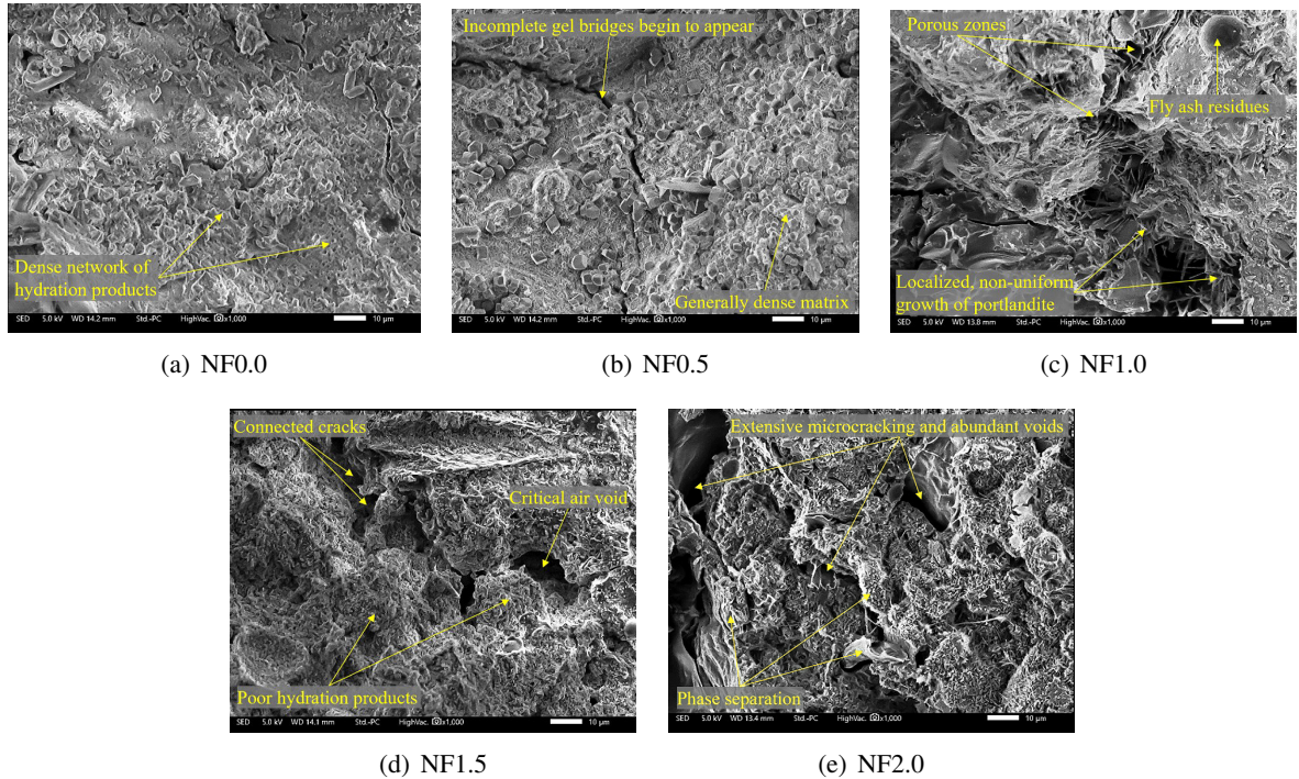
Figure 13. SEM micrographs of CC samples
