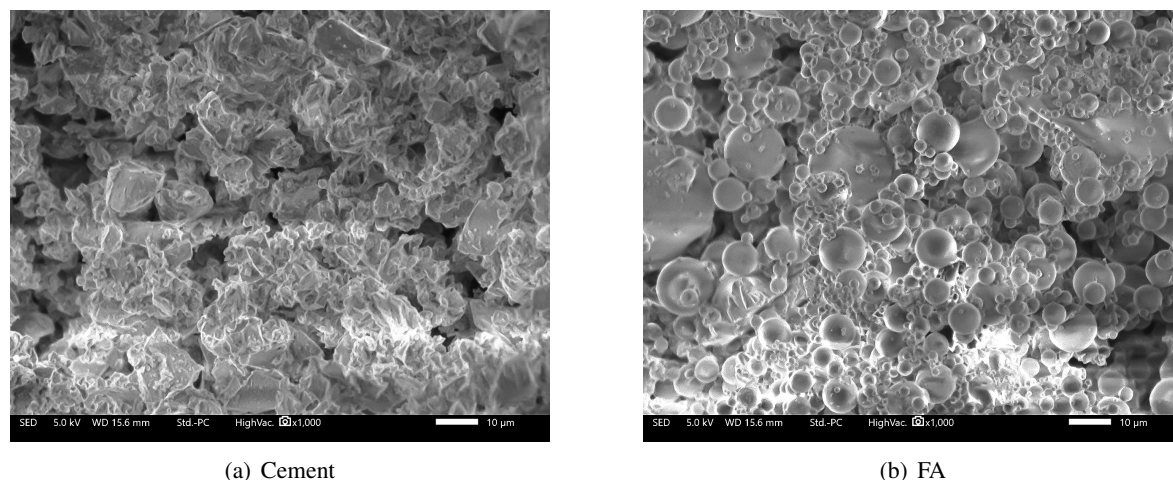
Figure 2. SEM images of cement and FA
