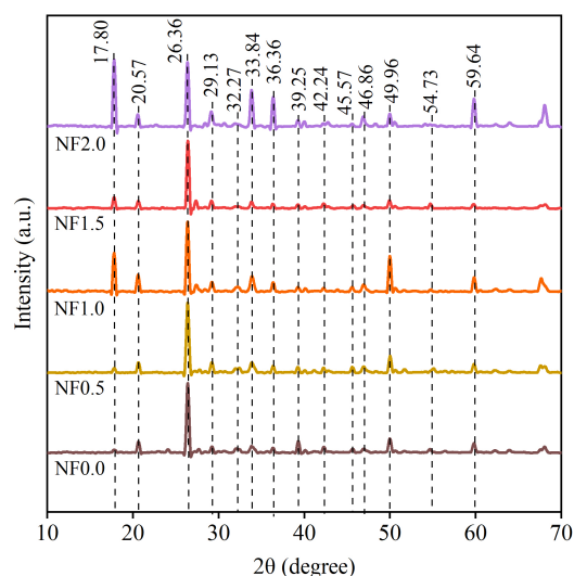
Figure 12. XRD patterns of CC samples
