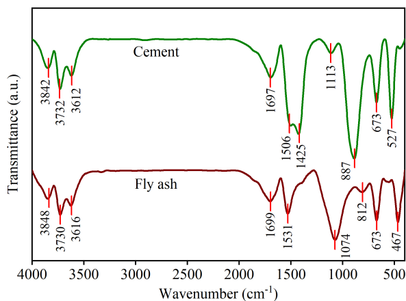
Figure 3. FTIR spectra of cement and FA
