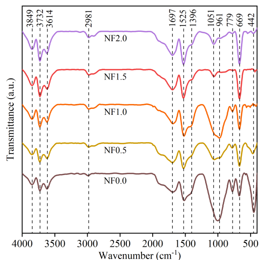
Figure 11. FTIR spectra of CC samples
