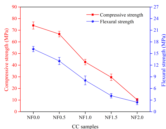
Figure 9. Mechanical strength of CC samples
