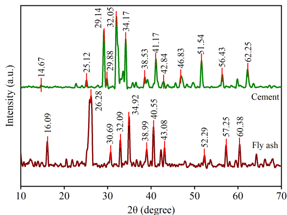
Figure 4. XRD patterns of cement and FA
