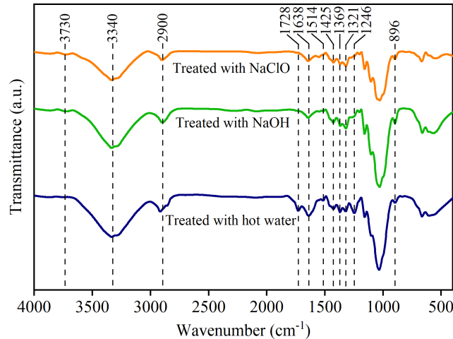
Figure 6. FTIR spectra of synthesized NFs
