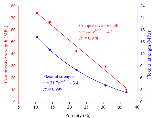
Figure 10. Correlation between porosity and mechanical strength of CC samples
