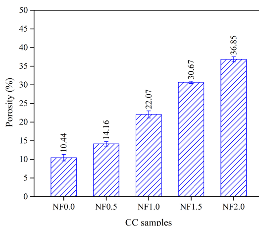
Figure 8. Porosity of CC samples
