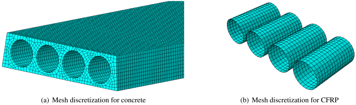
Figure 4. Mesh discretization of HC slabs for FEM
