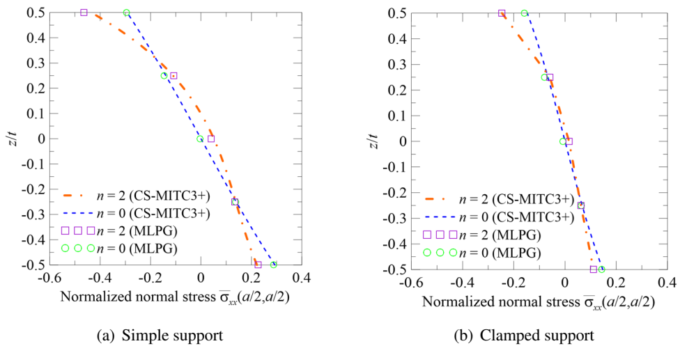
Figure 6. Variation of the normalized normal stresses through the thickness of the Al/ZrO 2 -1 plate with a/t = 5 under the uniformly distributed load
