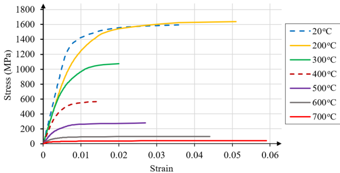
Figure 2. Engineering stress-strain ( \sigma_T - \epsilon_T ) curves of MS1200 steel sheets
