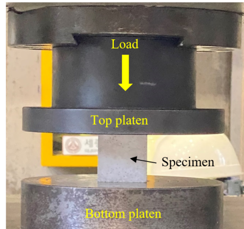
Figure 2. UTM used for compressive test
