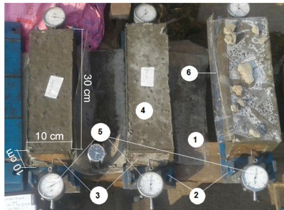
Figure 2. The mixing process and the measurement of plastic deformation of SCC specimens
