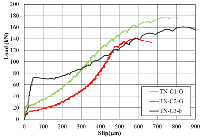
Figure 5. Load-slip curve
