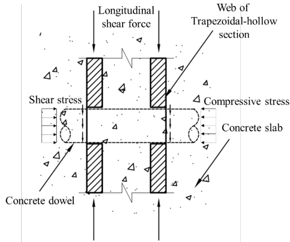
Figure 6. Stress state of concrete dowel
