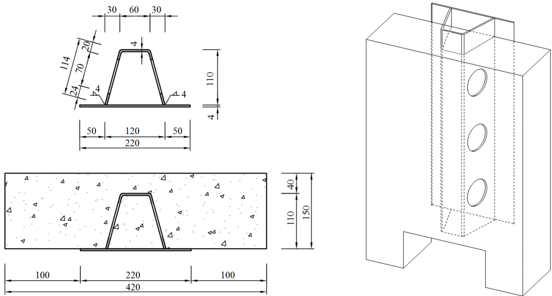
Figure 2. Dimensions and shape of push-out test specimens
