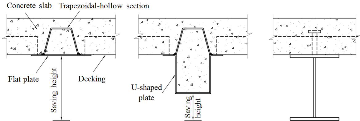
Figure 1. Cross-section of drawing of the shallow-hollow composite beam
